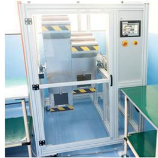
TUMBLE TEST 60 cycle, 0.5m height
